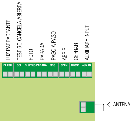
ROBUS 400/600/1000
