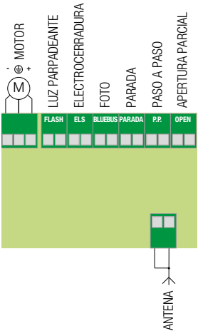
SLIGHT/NAKED SLIDING 400/ROBUS HS
